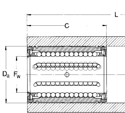
Linear bearing unit with seals
