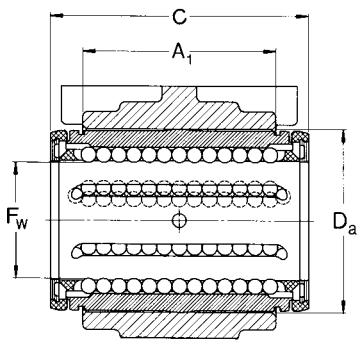
Linear bearing unit with 2 shields
