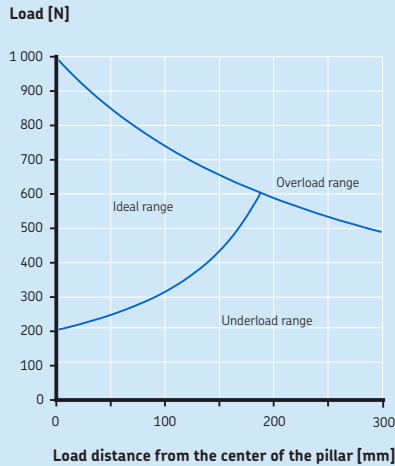
Offset load diagram CPMA1-1
