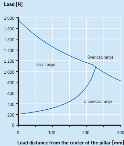
Offset load diagram CPMA1-2 and CPMA2-2
