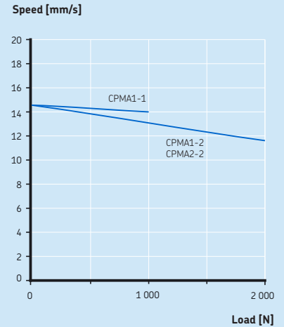
Speed-load diagram
